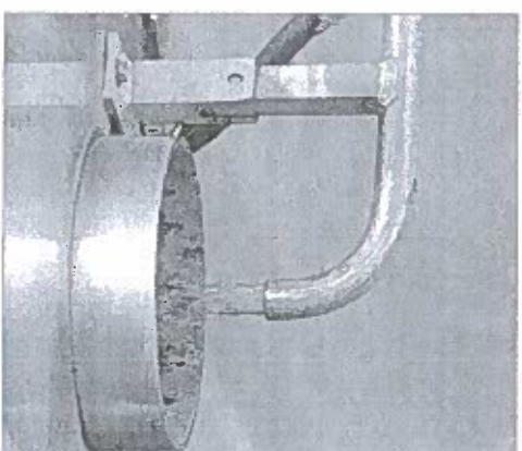
Figure 2-5. An air gap prevents back siphoning while filling a spray tank.
